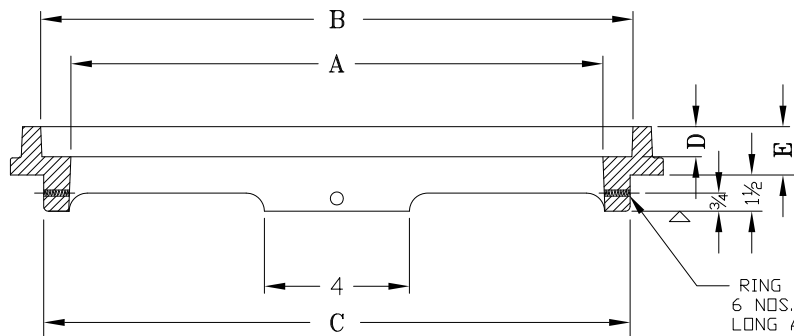
SECTION-X-X
