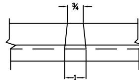
VIEW-Y-Y
