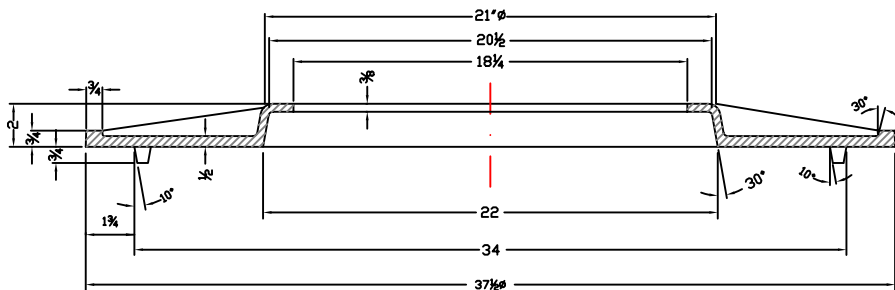
SECTION-X-X
