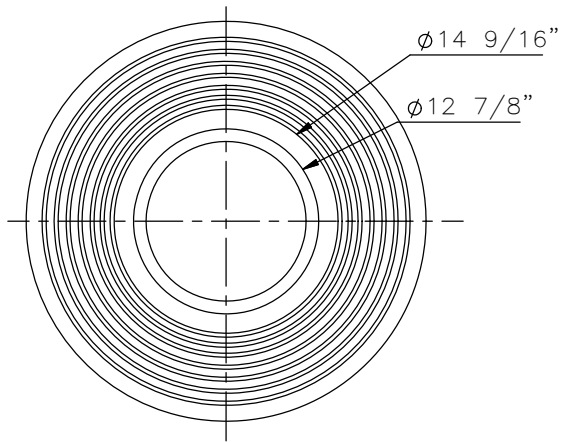
TOP VIEW OF OUTER LID
